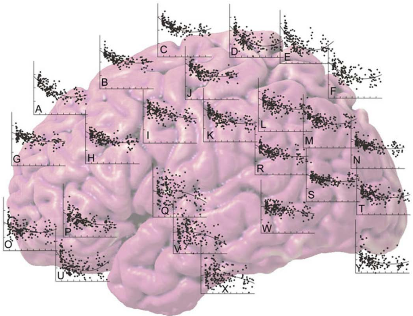
Fig. 1. Cortical thickness shows regional and temporal specificity with development (Sowell et al. 2003). Shown is a surface rendering of the left hemisphere of the brain (anterior to posterior is left to right ), with scatterplots of nonlinear relationship between gray matter density and age in years. Graphs are placed over the corresponding brain regions. All axes are identical; gray matter density is plotted on the x-axis, and age in years (range: 7–87 years) is plotted on the y-axis. Prefrontal and parietal regions show steeper or prolonged rates of decline compared to phylogenetically older regions like the occipital lobe. In contrast, temporal regions show increases in gray matter density before starting to decline in adolescence
