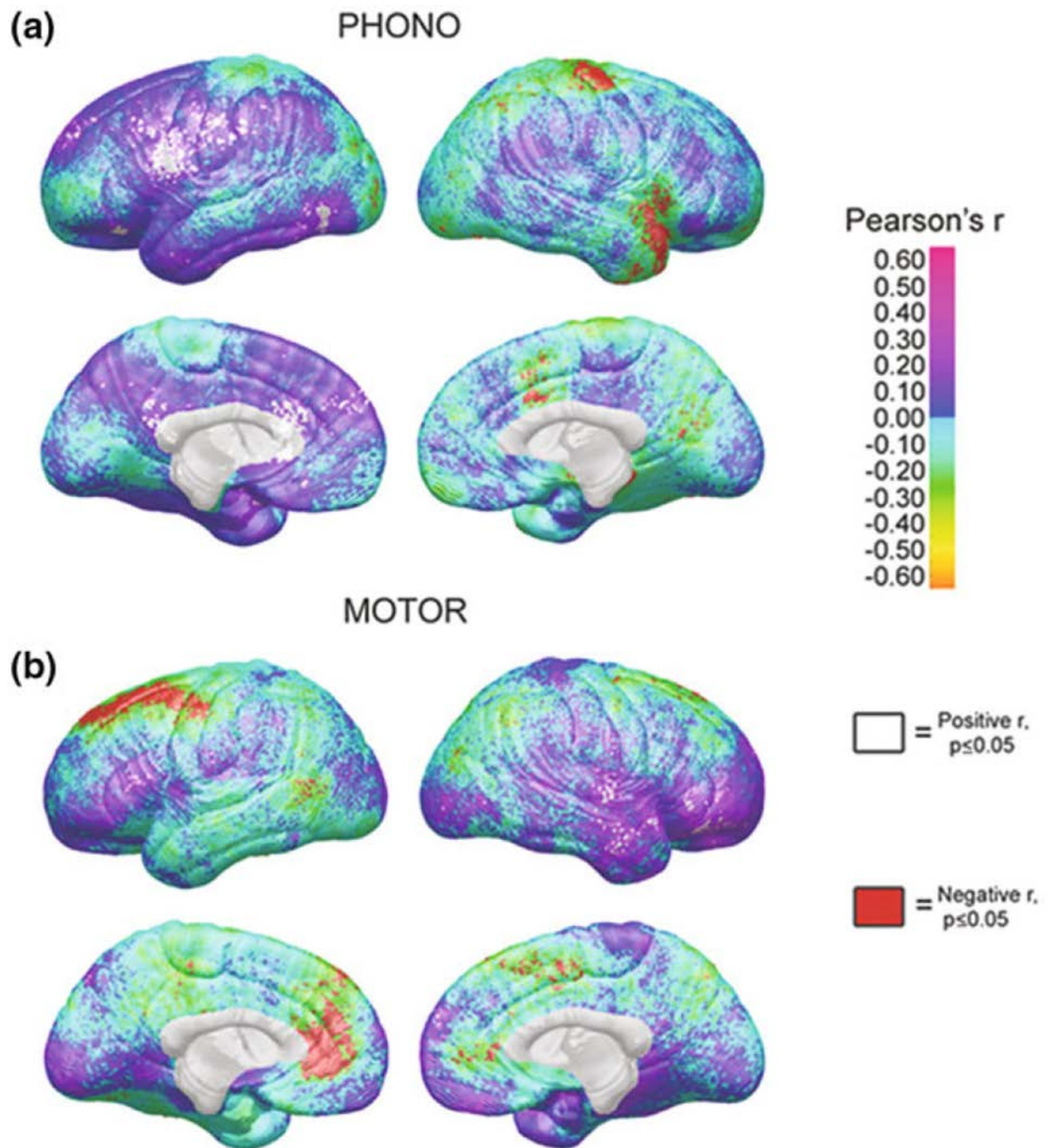
Fig. 2. Localized thickness maps of both cerebral hemispheres reveal Pearson's correlations ( p \leq 0.05 ) between changes in gray matter thickness and behavioral scores on a phonological processing, and b fine motor skill in children (ages 5–11 years). A double dissociation is seen between thickness and behavior, as white areas represent positive relationships between behavior and thickness change; red areas represent negative correlations (used with permission; Lu et al. 2007)
