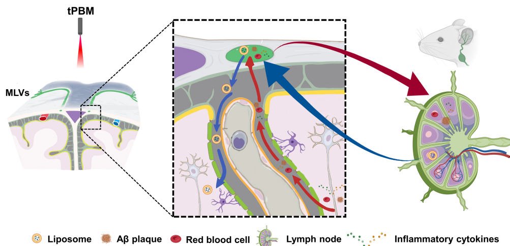
Fig. 4 Illustration of new tPBM strategy for brain disease treatment: red and blue arrows represent MLVs-mediated toxins evacuation pathway and liposome-loaded drug delivery pathway, respectively. Some items were created with BioRender.
